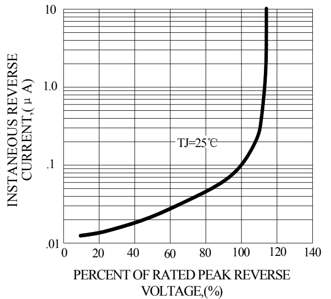
FIG.4-TYPICAL REVERSE CHARACTERISTICS
